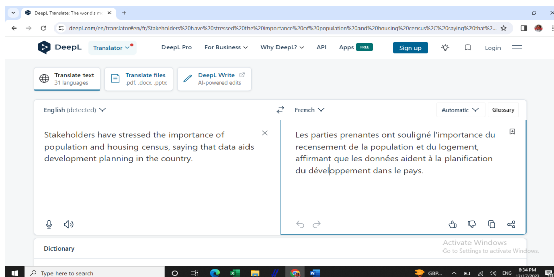
Figure 1: DeepL environment.
